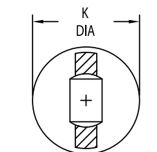
SECTION X-X (BOLT PLATE SIZE 1/4-10)
